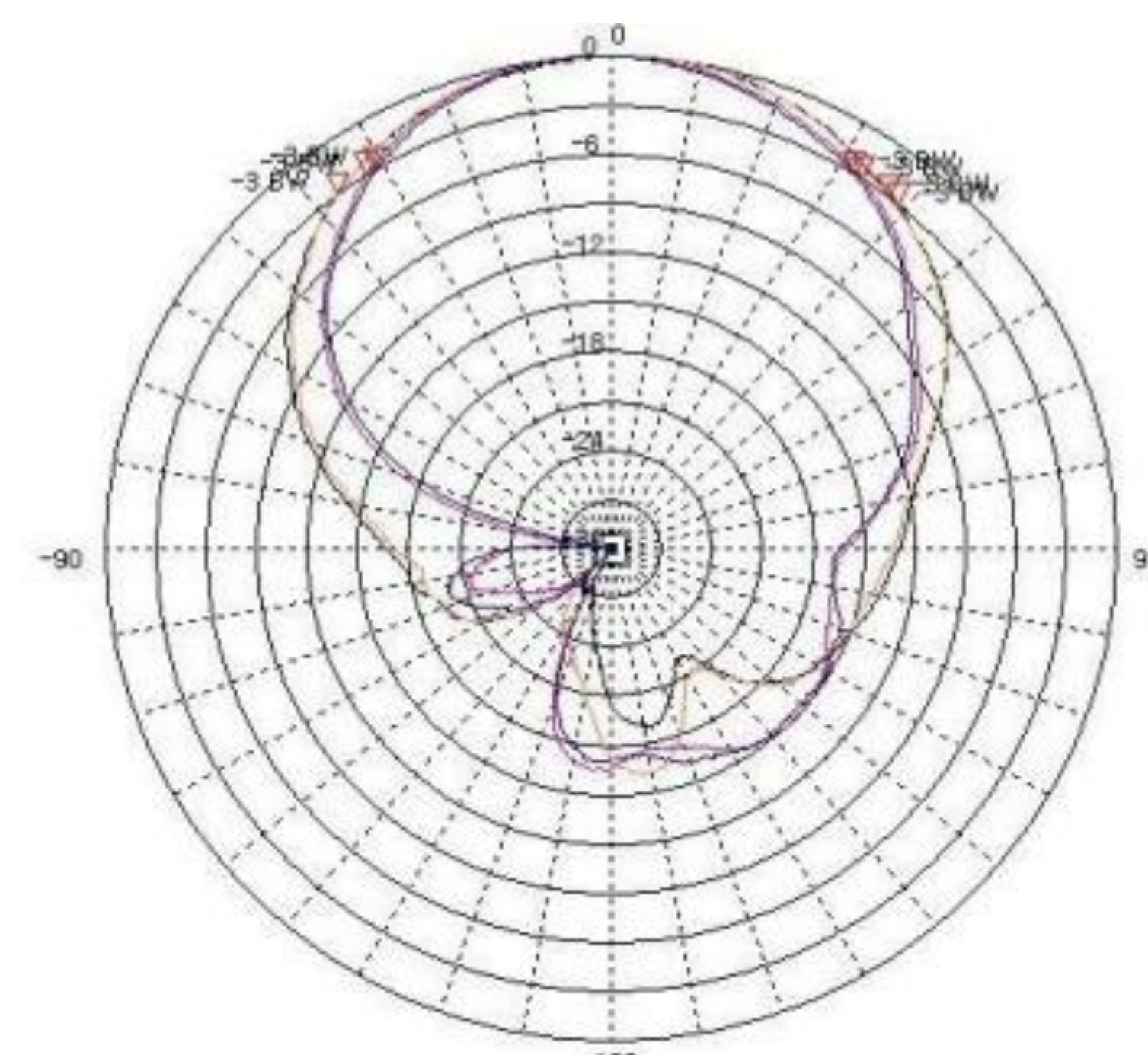
Vertical Pattern
